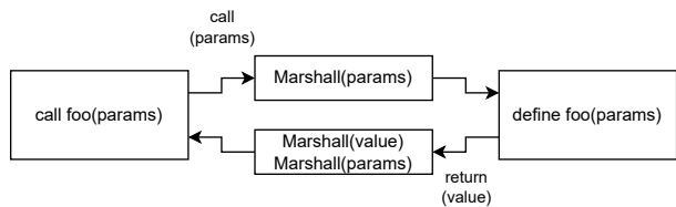
Figure 3. Marshalling When Invoking a Foreign Function
